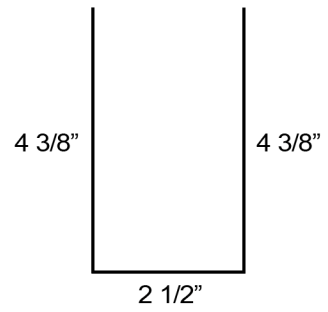
Wire Bending Diagram (Not to scale)
